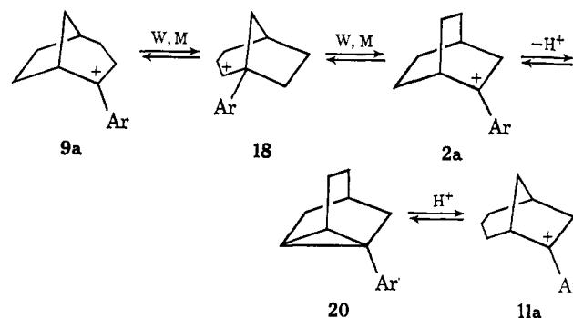
Scheme V
