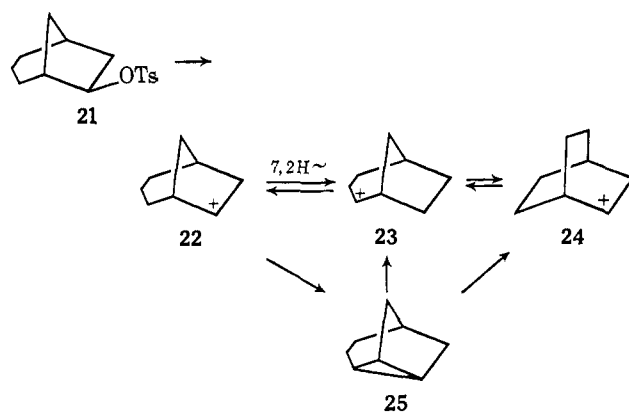
Scheme V
